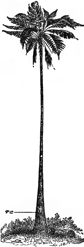
EAST INDIA TREE-FERN.* ( Asophila perrotetiana. )
